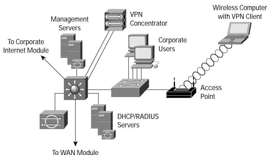
Figure 8 Medium Network VPN WLAN Design
